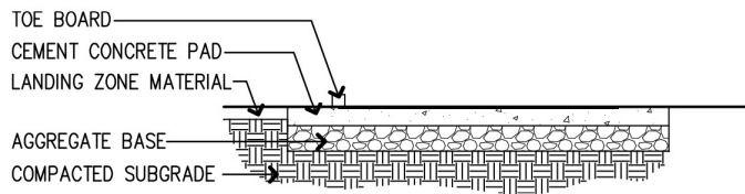
SHOT PUT PAD SECTION A-A
