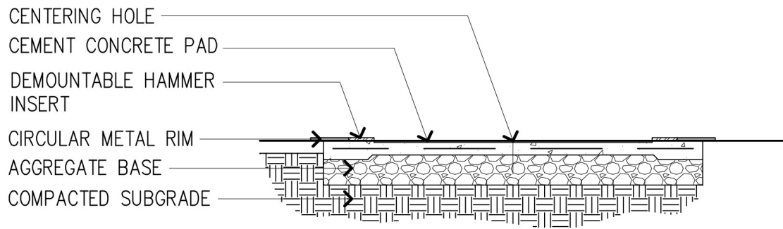
DISCUS/HAMMER PAD SECTION A-A
