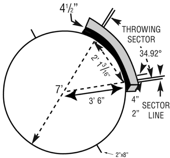
SHOT PUT PAD PLAN VIEW
